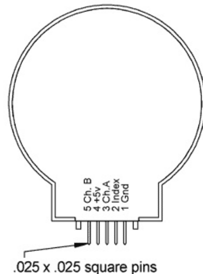
US Digital Encoder (S2 series)
